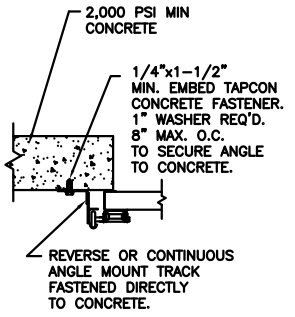
CONCRETE JAMBS
