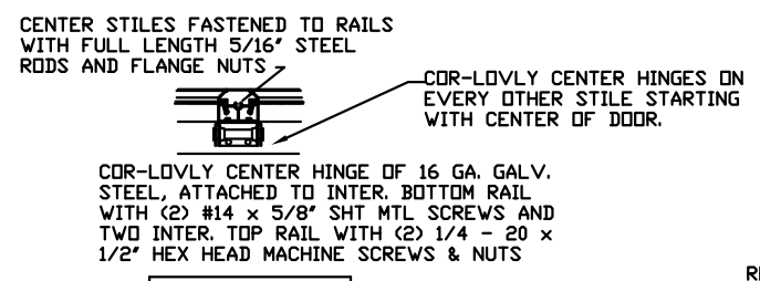
SECTION 2-2
