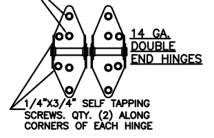
VIEW "A"
