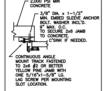
WOOD JAMB ON CONCRETE
