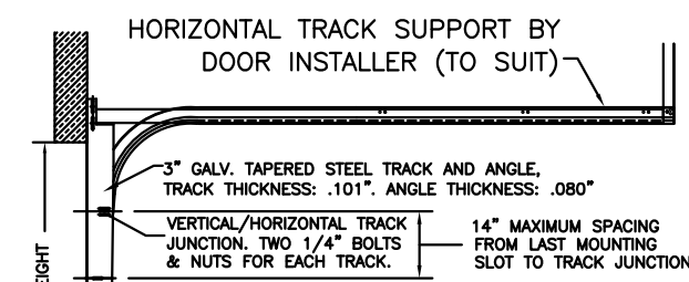
TRACK CONFIGURATION
