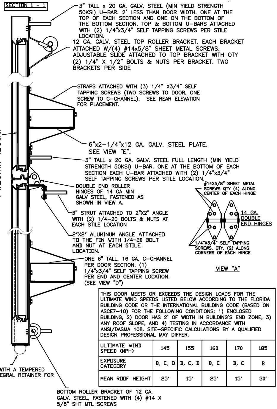
SECTION 1-1
