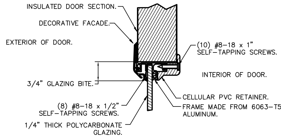
IMPACT-RESISTANT ASSEMBLY DETAILS DRAWING 104801-A
