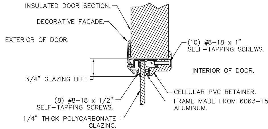
IMPACT-RESISTANT GLAZING DETAILS
