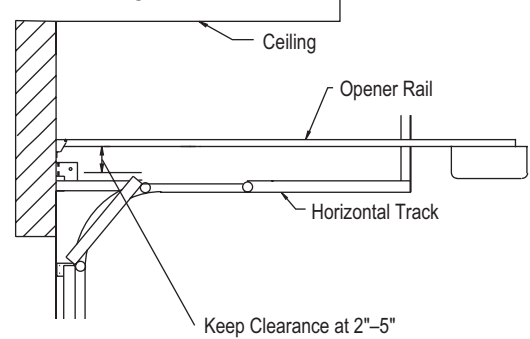
Opener Rail Mounting Distance
