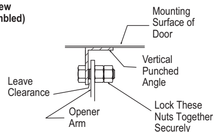
Fig. 15-D (Doors with angle iron reinforcement bracket and stile in center of door)
