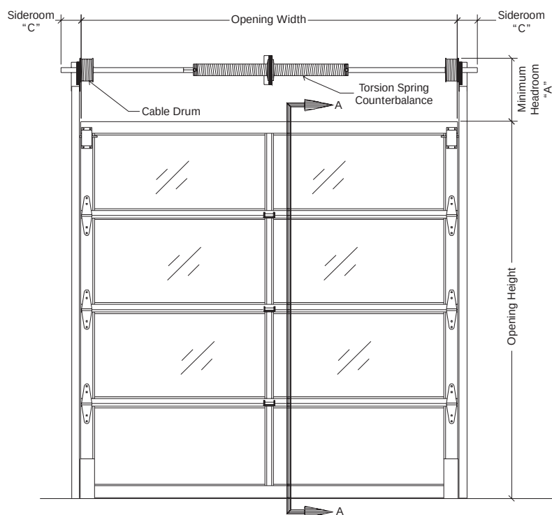
INTERIOR ELEVATION
