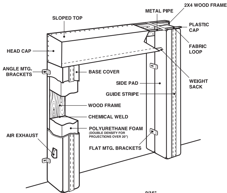
REINFORCED INSIDE
