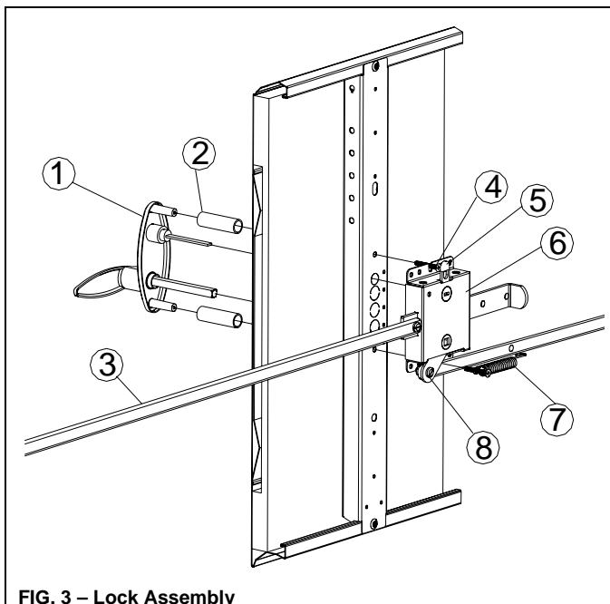
FIG. 3 – Lock Assembly
