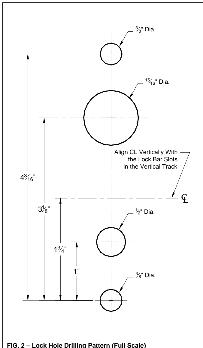
FIG. 2 – Lock Hole Drilling Pattern (Full Scale)
