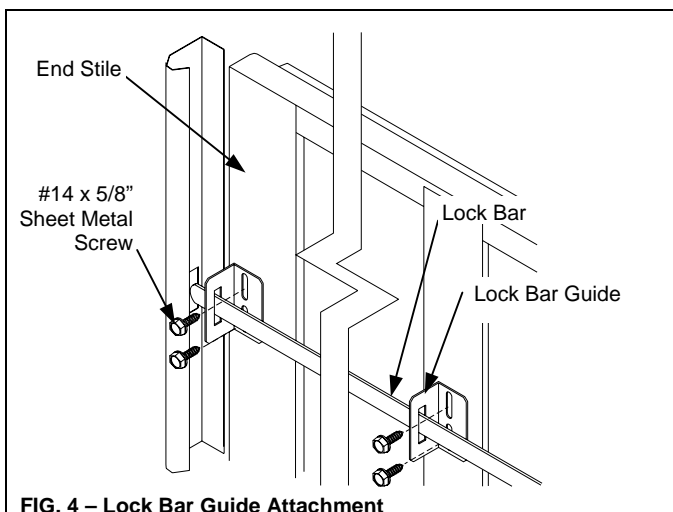
FIG. 4 – Lock Bar Guide Attachment
