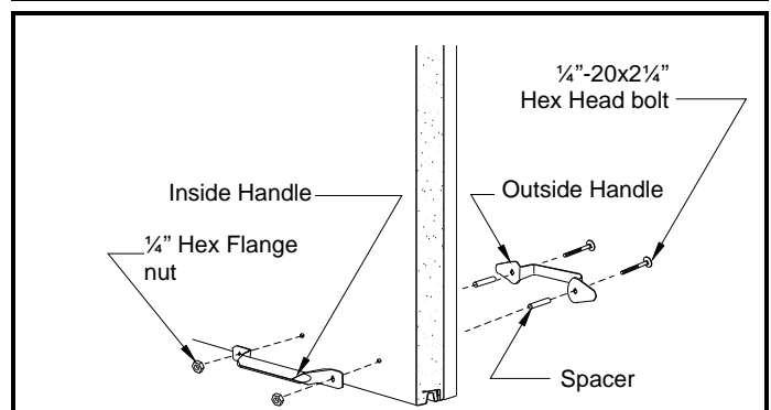
FIG. 8 – Lower Lift Handle Attachment
