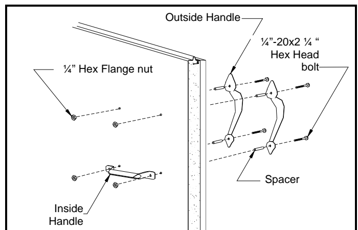
FIG. 9 – Upper Lift Handle Attachment
