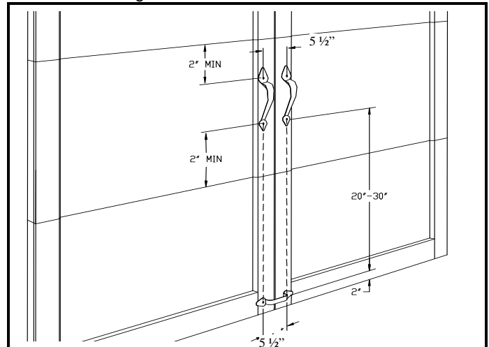
FIG. 7 – Outside Lift Handle Placement
