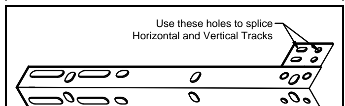
FIG. 10 – Flag Bracket for Premium Models
