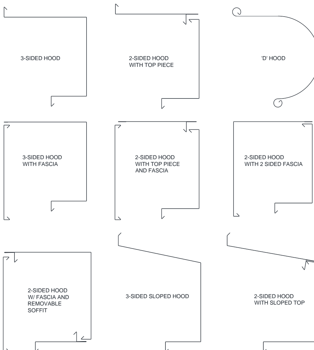
Figure 11.1 - Hood Configurations
